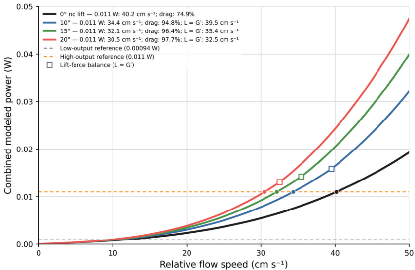
Fig. 4 Combined modeled power versus relative flow speed for the streamlined no-lift baseline and the lift-adjusted 10^\circ , 15^\circ and 20^\circ scenarios.
