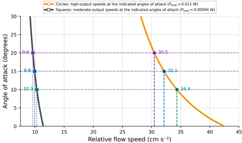
Fig. 3 Modeled relationship between angle of attack and the relative flow speed at which lift-adjusted total power—comprising apparent-weight-related and hydrodynamic-drag components—reaches the modeled moderate-output (0.00094 W; gray curve) and high-output (0.011 W; orange curve) values. Squares and circles identify the respective moderate- and high-output intersection speeds at the illustrative 10°, 15°, and 20° angles of attack; adjacent values are speeds in \text{cm s}^{-1} .
