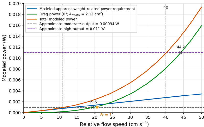
Fig. 2 Modeled power requirements for W. trifurcatus as functions of relative flow speed in the streamlined 0° position. Curves show the apparent-weight-related requirement, the power required to overcome hydrodynamic drag, and their sum. Dashed lines and markers identify the approximate moderate- and high-output values and the modeled hydrodynamic transition conditions described in the text.
